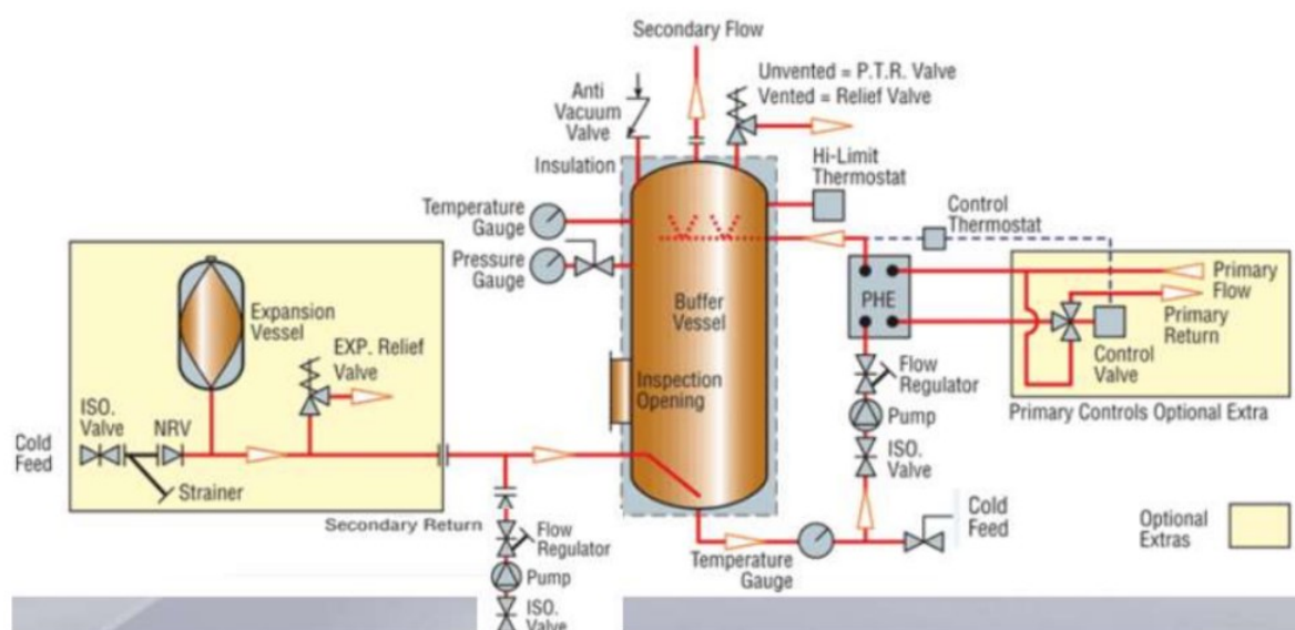
Figure 17. Typical schematic layout of a calorifier and expansion vessel 112 .
